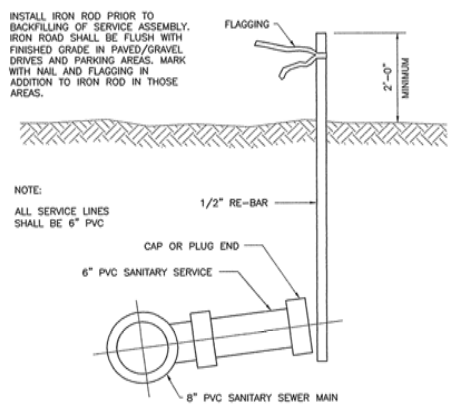
SERVICE CONNECTION DETAIL N.T.S.
