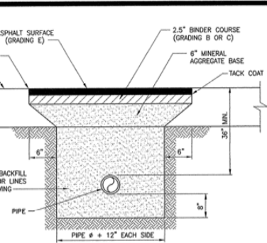
SPECIAL DETAIL PAVEMENT CUT-ASPHALT N.T.S.
