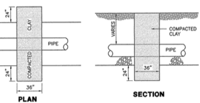
COMPACTED CLAY CHECK DAM N.T.S.
